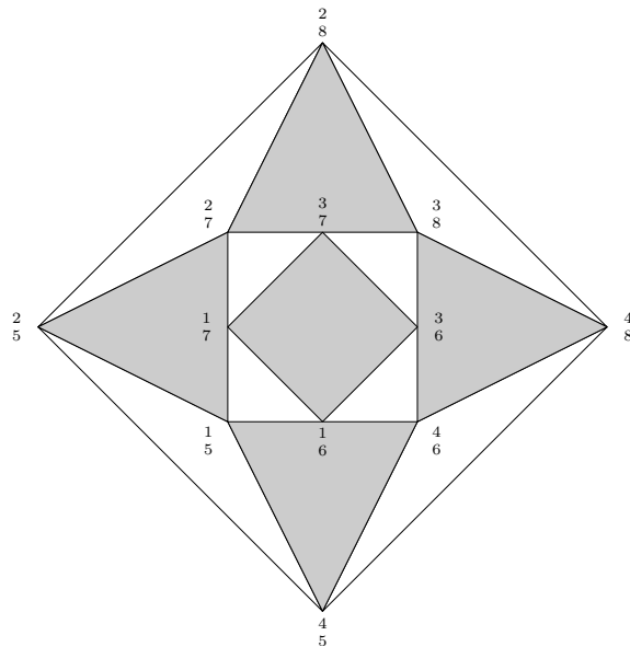
Figure 10. Separating sphere of an 8-vertex cylinder S^2_4 \times [0, 1] - A cuboctahedron (drawn as a Schlegel diagram of a quadrilateral face).
